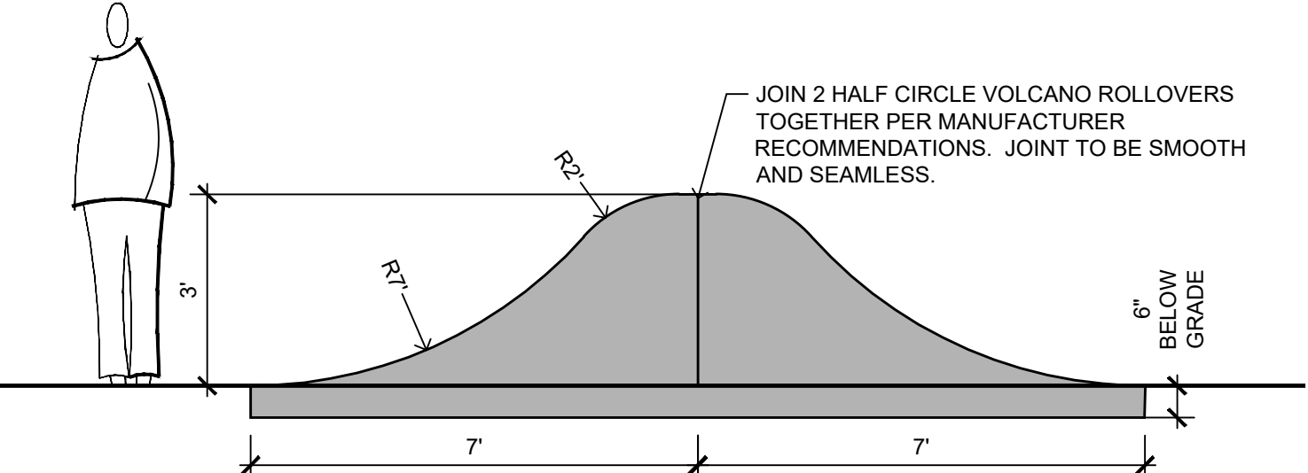
6 PARK A LS503 ELEVATION: SKATE FEATURE - VOLCANO ROLLOVER NTS
