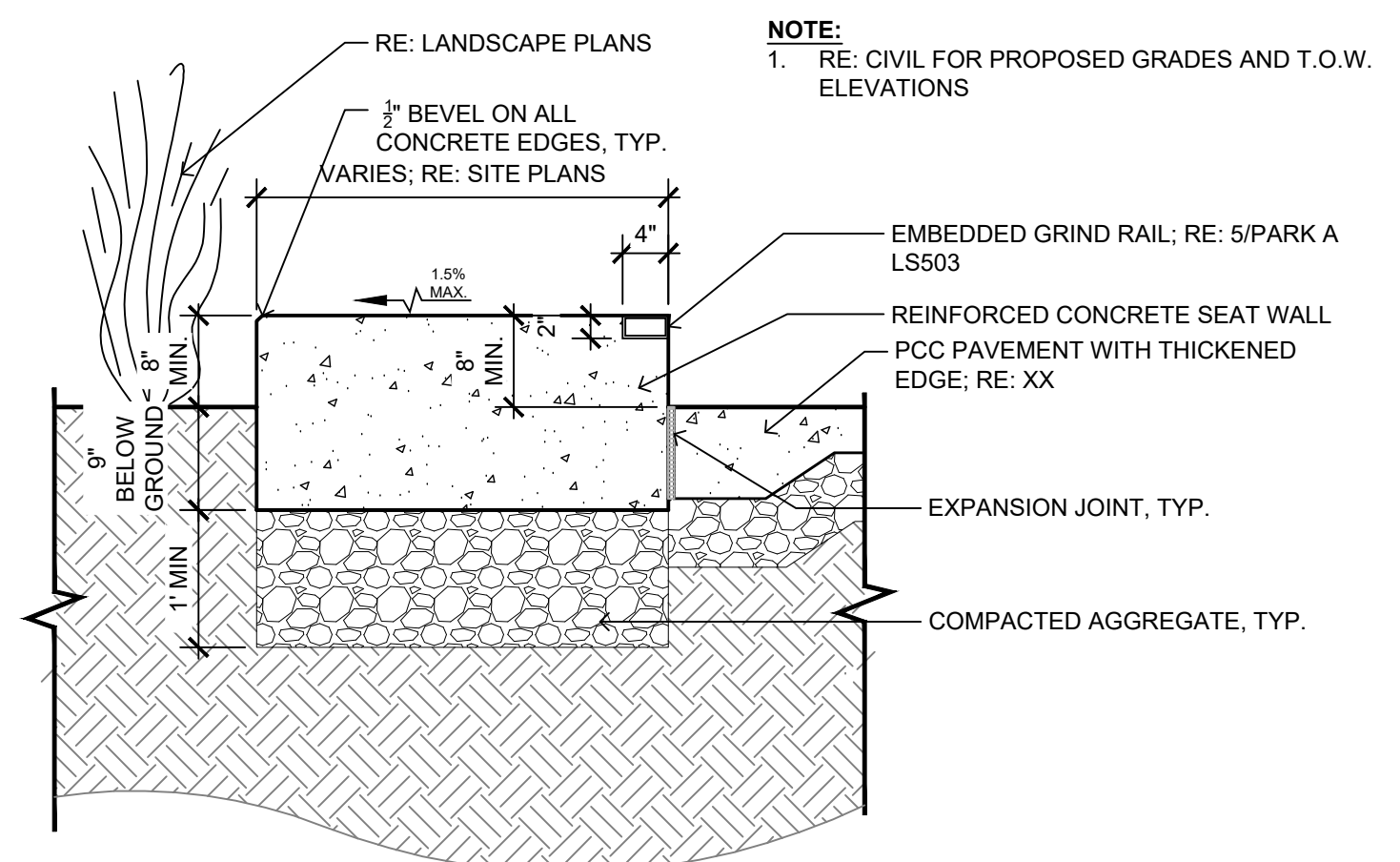
2 PARK A LS503 SECTION: SKATE WALL (8" HT.) 3/4" = 1'-0"
