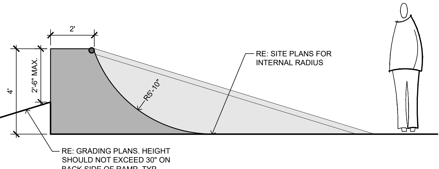
7 PARK A LS503 ELEVATION: SKATE FEATURE - CURVED TACO 3/8" = 1'-0"
