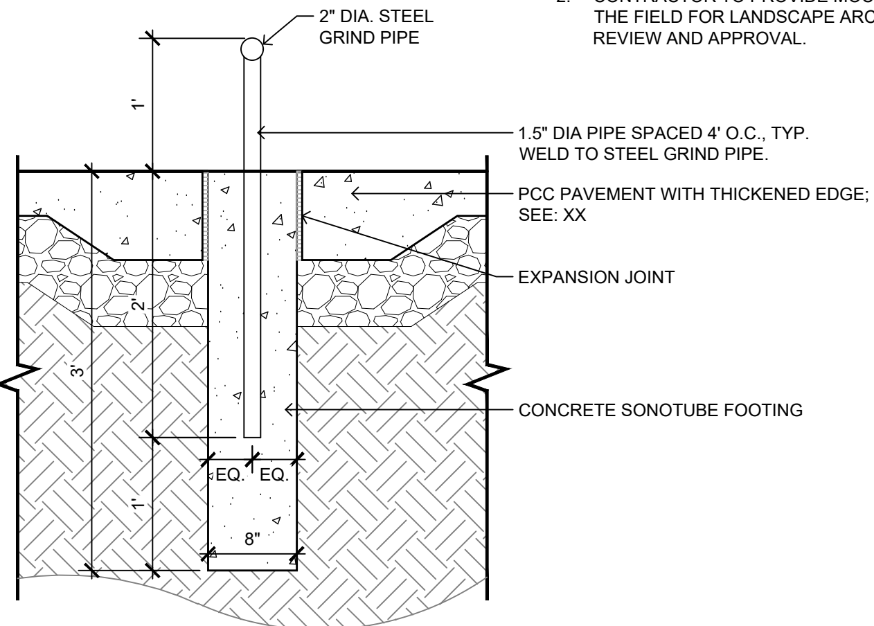
10 PARK A LS503 SECTION: SKATE RAIL 1" = 1'-0"
