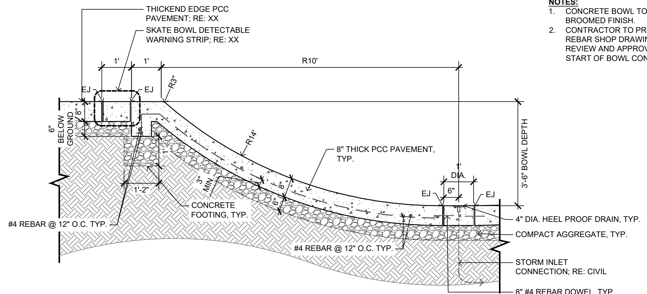
2 PARK A LS504 SECTION: SKATE BOWL (10' RADIUS) 1/2" = 1'-0"
