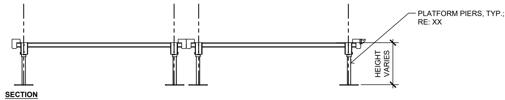
02 PARK A LS502 DETAIL: PLATFORM DECKING 1/2" = 1'-0"
