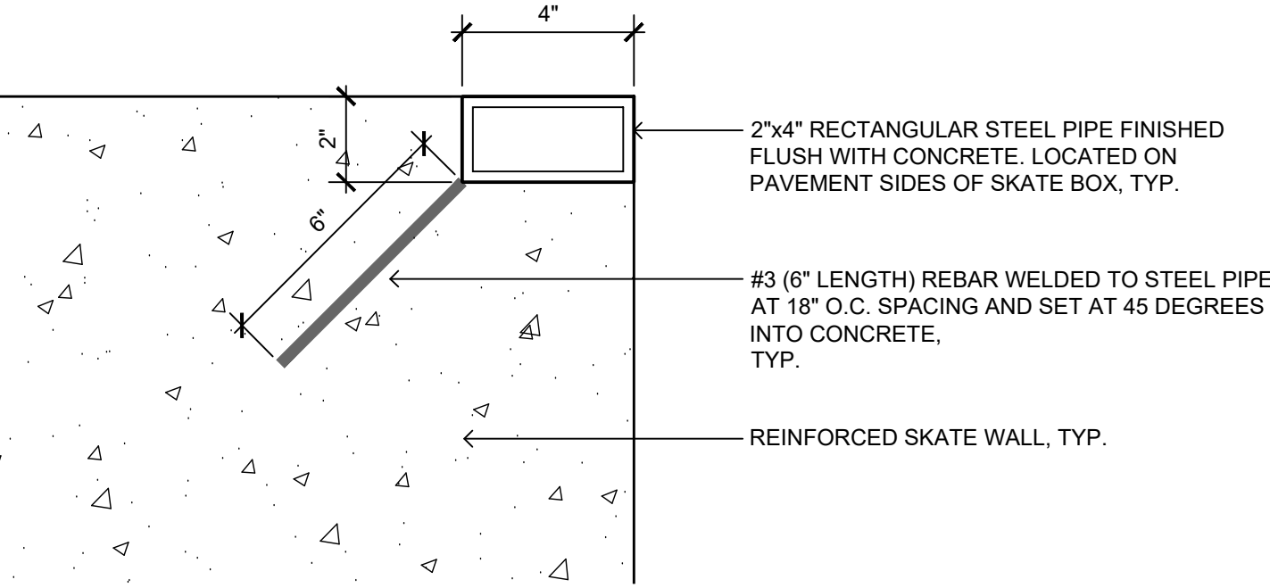
5 PARK A LS503 SECTION: EMBEDDED GRIND RAIL, TYP. NTS
