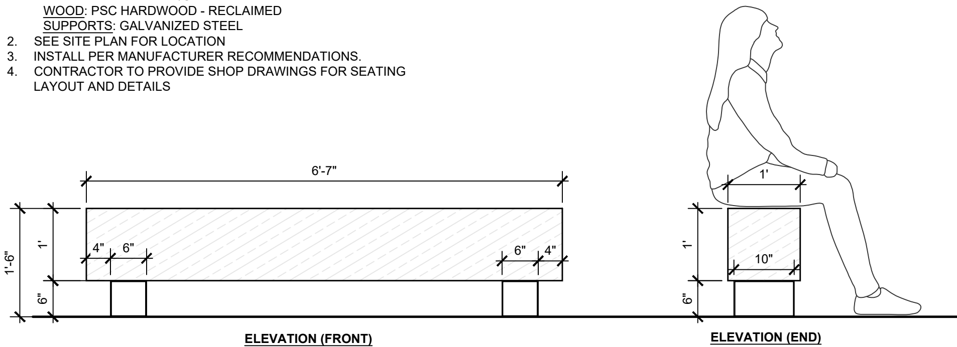
04 PARK A LS502 DETAIL: LOG SEATS AT VIEWING PLATFORM 3/4" = 1'-0"
