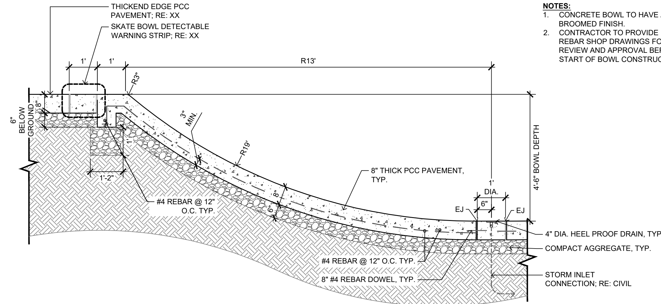
3 PARK A LS504 ELEVATION: SKATE BOWL (13' RADIUS) 1/2" = 1'-0"
