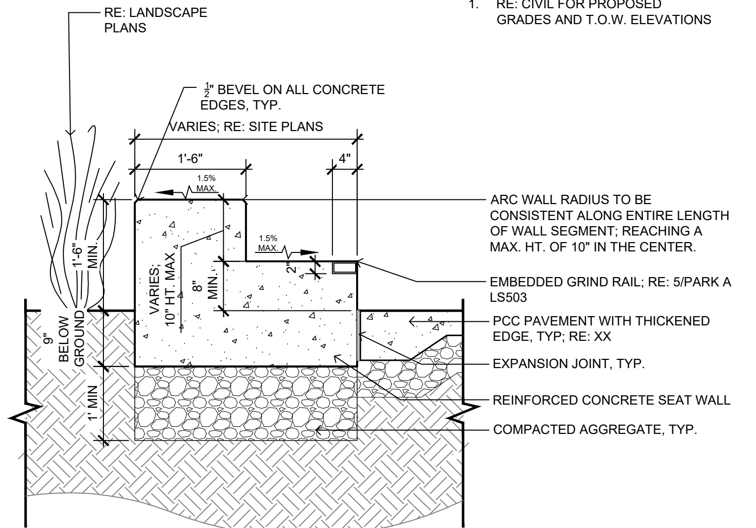
4 PARK A LS503 SECTION: SKATE WALL (8" HT. WITH ARC WALL SEGMENT) 3/4" = 1'-0"
