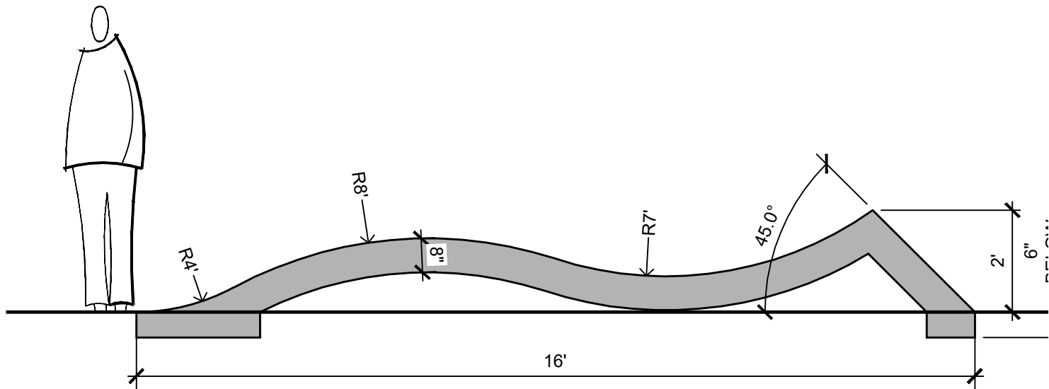
8 PARK A LS503 ELEVATION: SKATE FEATURE - ROLLOVER WHIP NTS
