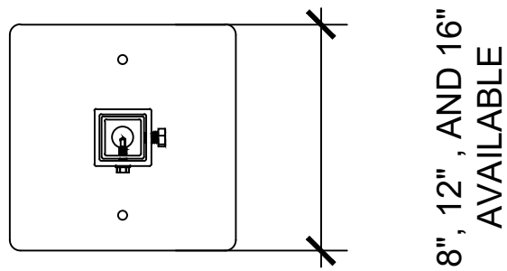
03 PARK A LS502 DETAIL: PLATFORM PIERS 3/4" = 1'-0"
