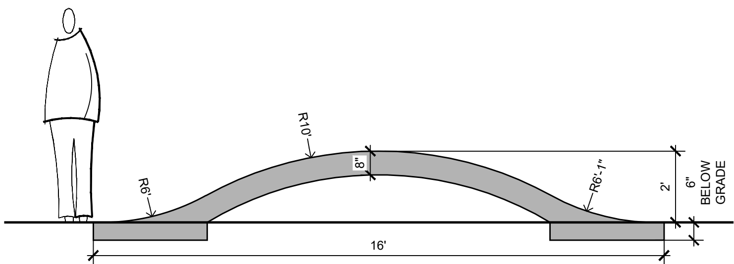
9 PARK A LS503 ELEVATION: SKATE FEATURE - ROLLER COASTER NTS
