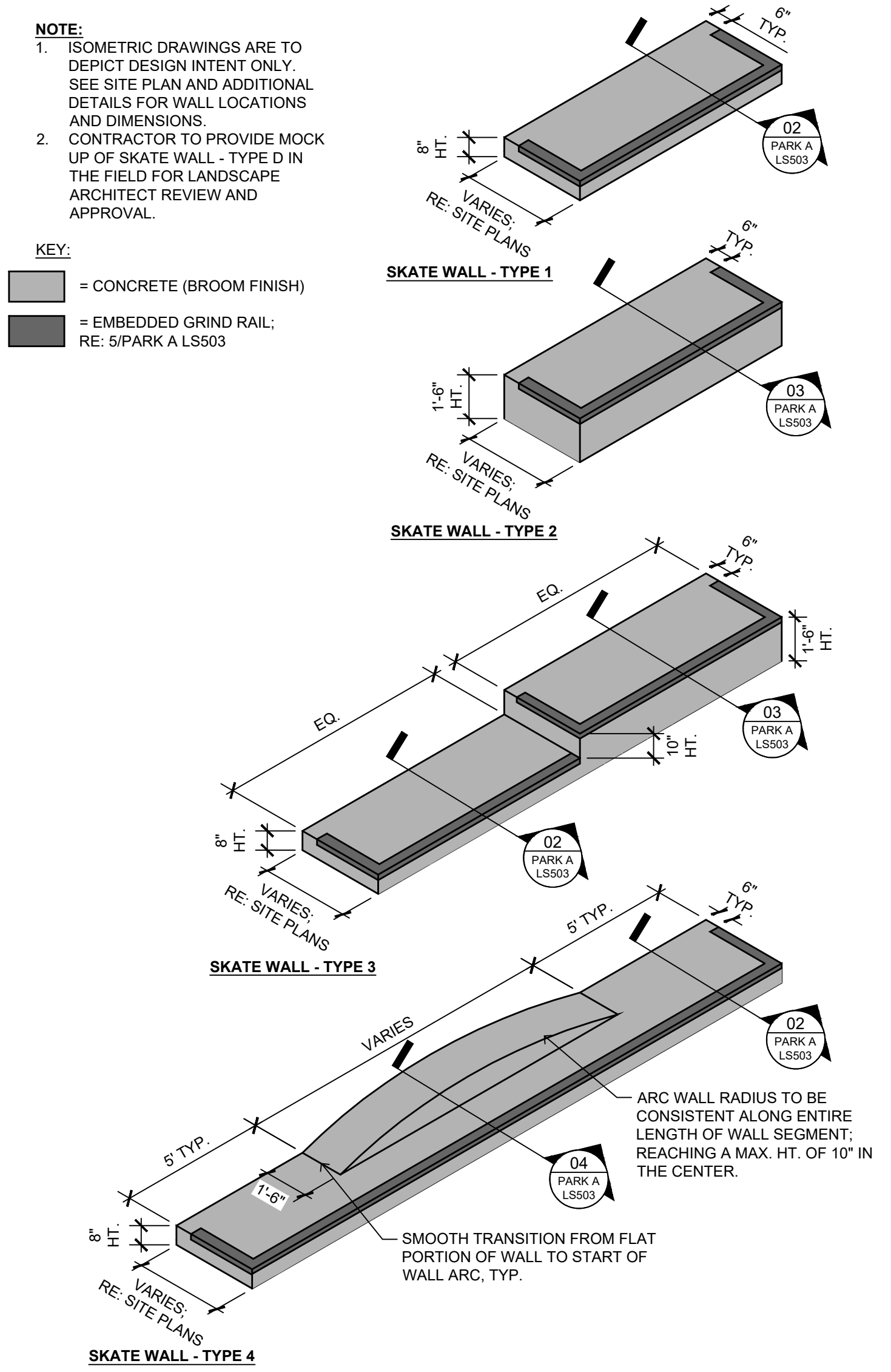
1 PARK A LS503 DETAIL: TYPICAL SKATE WALL TYPES NTS
