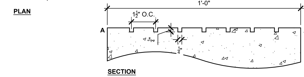
4 PARK A LS504 SECTION: SKATE BOWL DETECTABLE WARNING STRIP 1" = 1'-0"
