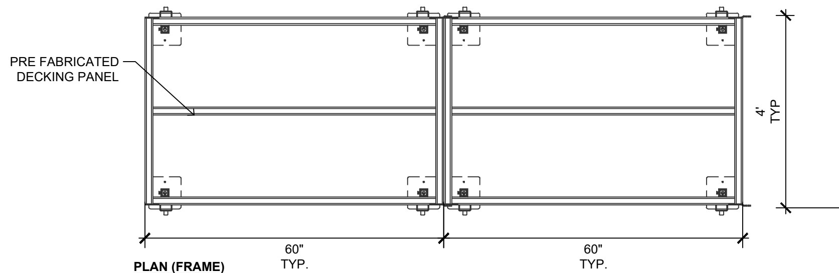
PLAN (FRAME)
