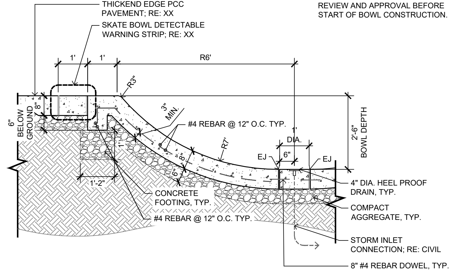
1 PARK A LS504 SECTION: SKATE BOWL (6' RADIUS) 1/2" = 1'-0"
