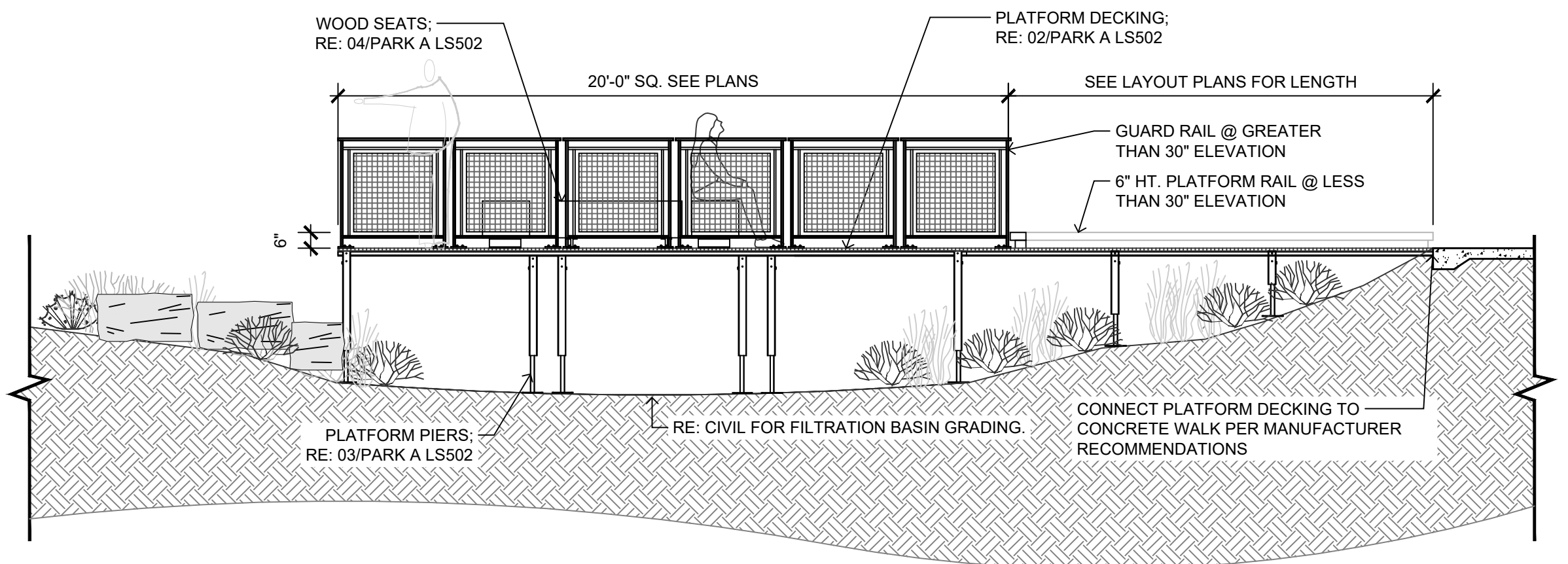
01 PARK A LS502 SECTION: BOARDWALK DECK & PLATFORM NTS
