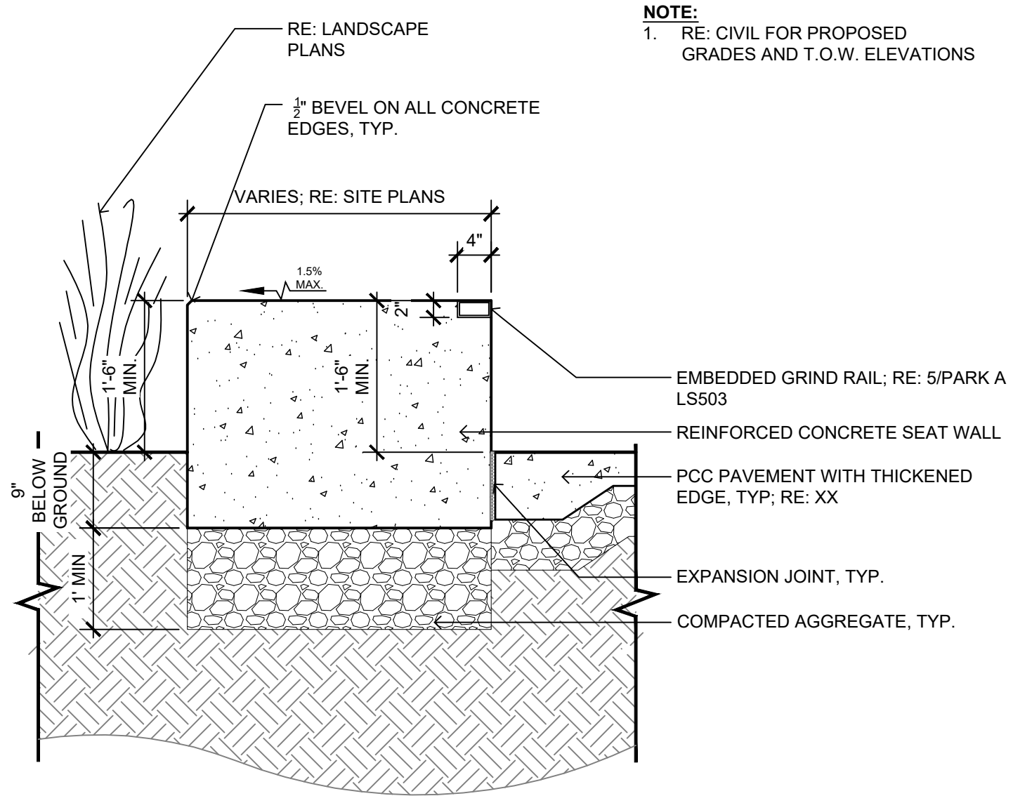
5 PARK A LS503 SECTION: EMBEDDED GRIND RAIL, TYP. NTS
