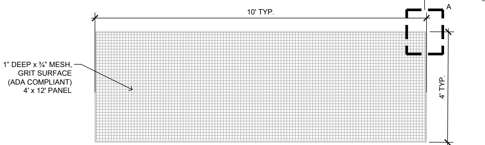
PLAN (GRATE)
